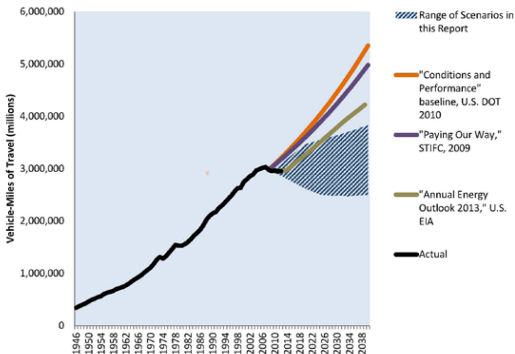
Figure 10. Recent Government Forecasts Compared with the Three Scenarios of VMT, 1946-2040
