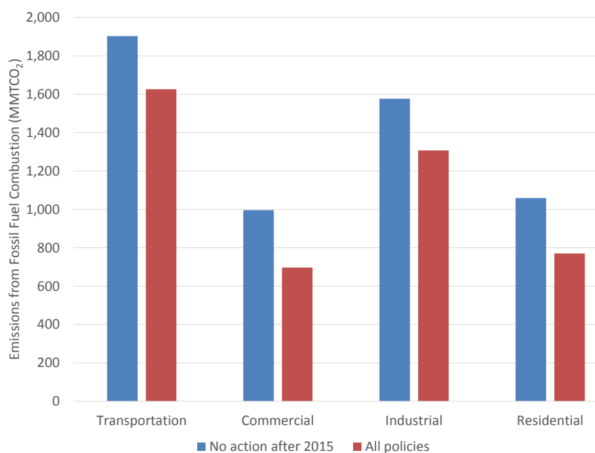
Figure 4. Carbon Dioxide Emissions in 2025 by Source of Energy Use (Including Electricity Consumption)
