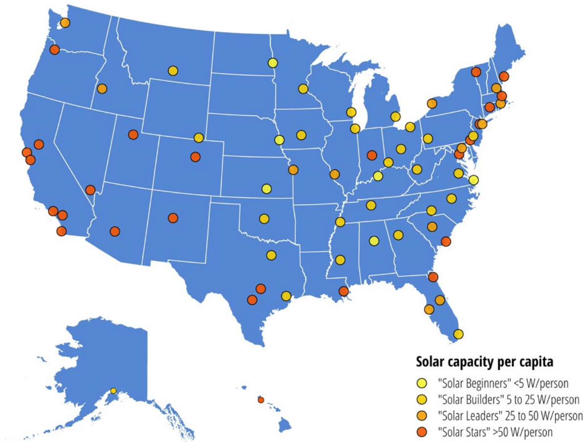
Figure ES-2. Major U.S. cities by installed solar PV capacity per capita, end of 2019 (watts per person)
