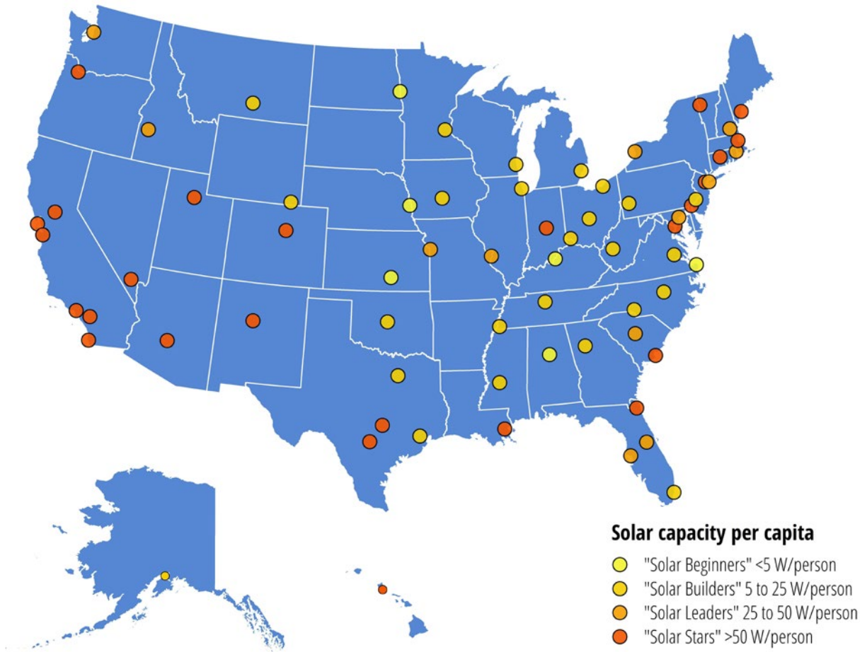
Figure 1. U.S. cities by installed solar PV capacity per capita, end of 2019 (watts per person)
